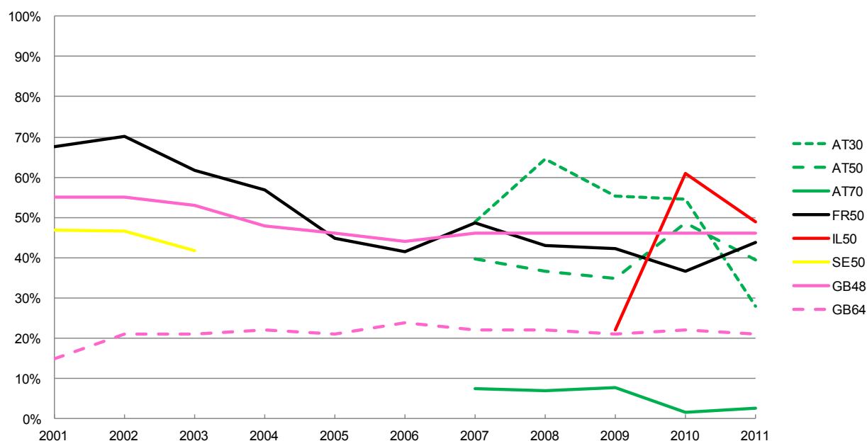
Fig. 10 Percentage of goods vehicles over 3.5 tonnes exceeding the speed limit on urban roads.
