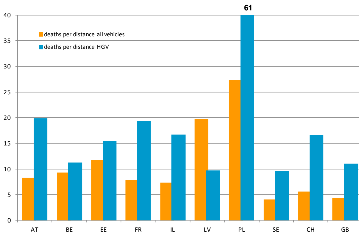
Fig. 4 Road deaths in collisions involving a goods vehicle over 3.5 tonnes per billion vehicle kilometres travelled by those vehicles (blue bars) with corresponding rates for all vehicles (orange bars). Average for the period 2008-2010 except for LV and SE 2009-2011 and PL 2008-2009.
