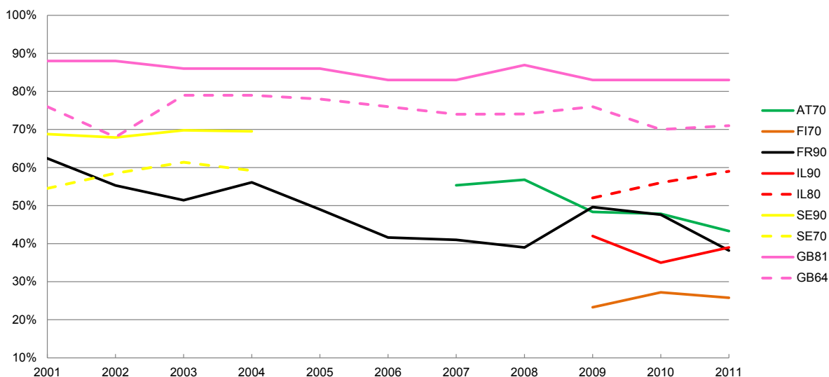
Fig. 8 Percentage of goods vehicles over 3.5 tonnes exceeding the speed limit on rural roads other than motorways.
