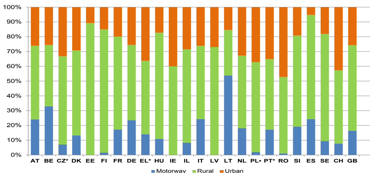
Fig. 3 Percentages by type of road of deaths in collisions involving a heavy goods vehicle in the last two or three years for which numbers are available (2009-2011 unless otherwise indicated).
