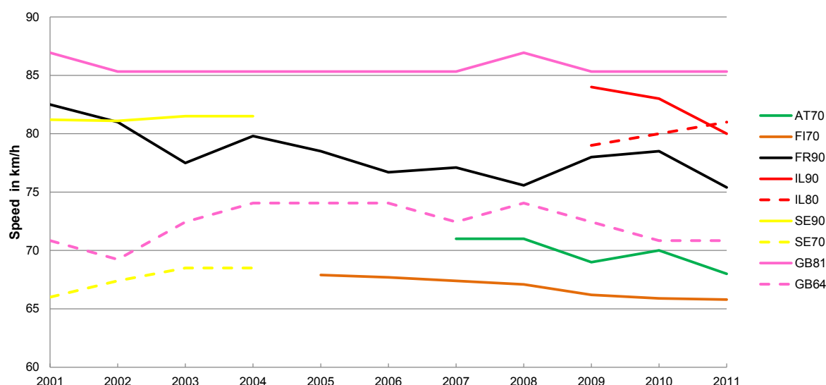
Fig. 7 Mean speed (in km/h) of goods vehicles over 3.5 tonnes, measured in free flowing traffic, on rural roads other than motorways in some European countries.
